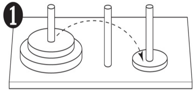
First move: Move disc 1 to peg 3.
