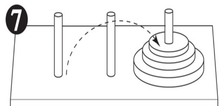
Seventh move: Move disc 1 to peg 3.
