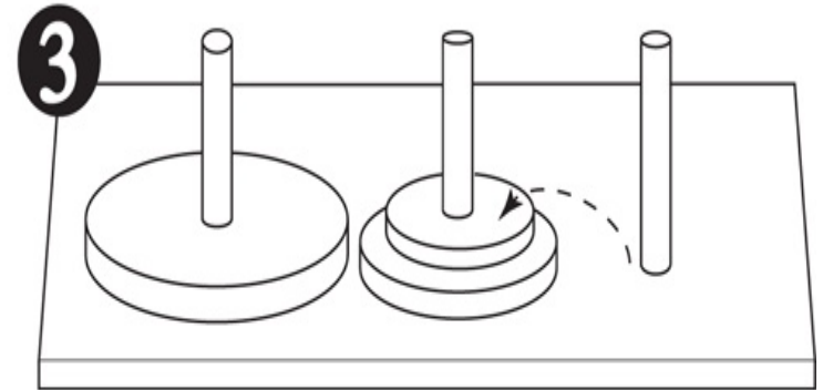
Third move: Move disc 1 to peg 2.
