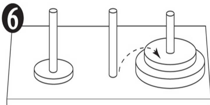
Sixth move: Move disc 2 to peg 3.
