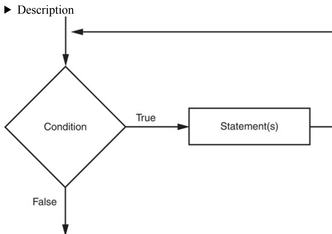
Figure 4-1 The logic of a while loop
