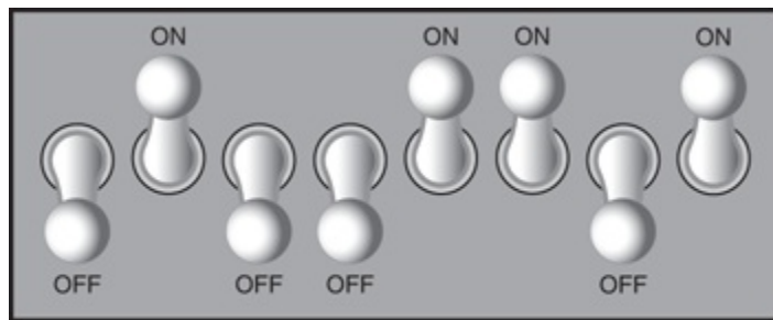
The number 77 stored in a byte.
