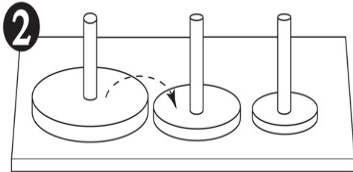
Second move: Move disc 2 to peg 2.
