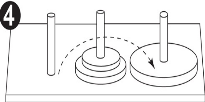
Fourth move: Move disc 3 to peg 3.
