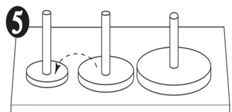
Fifth move: Move disc 1 to peg 1.
