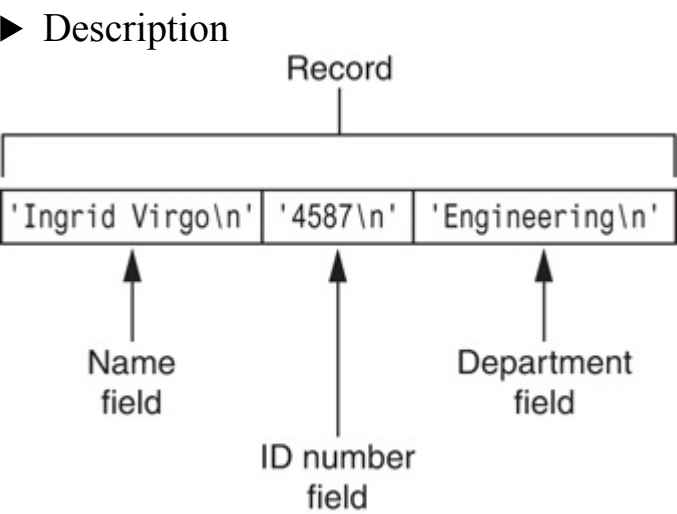
Figure 6-18 Fields in a record
